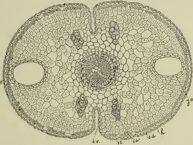
FIG. 75.—Savin, transverse section of twig. ca , cells with bordered pits; ed , epidermis of lower surface of adnate leaf; ev , epidermis of upper surface; go , oil gland; h , hypodermis; st , stoma. (Collin.)
